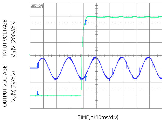
Figure 5. Typical Start-up ( V_{IN} = 115\text{Vac} ).
