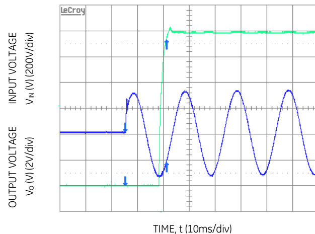
Figure 6. Typical Start-up ( V_{IN} = 230\text{Vac} )
