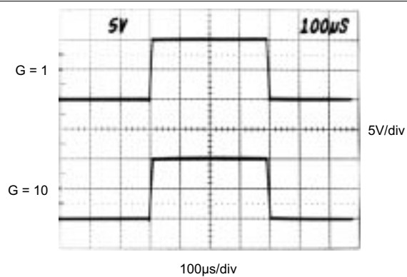
Figure 7-23. Large-Signal Response
